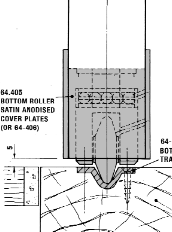
SECTION-TIMBER FLOOR
