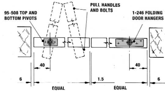
PLAN SHOWING TWO LEAVES FOLDING TO ONE SIDE
