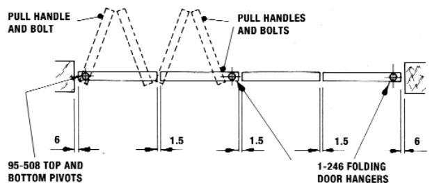
PLAN SHOWING FOUR LEAVES FOLDING TO ONE SIDE
