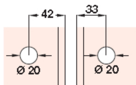
Glass machining without miter, 8 mm glass
