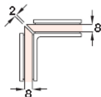
Glass machining with 45° miter, 8 mm glass
