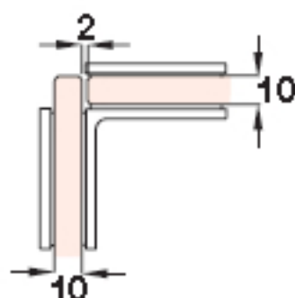
Glass machining without miter, 10 mm glass
