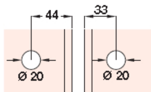
Glass machining without miter, 10 mm glass
