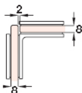
Glass machining without miter, 8 mm glass
