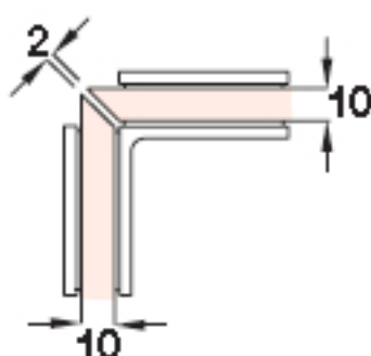
Glass machining with 45° miter, 10 mm glass
