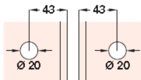
Glass machining with 45° miter, 10 mm glass
