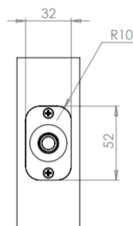
Face Plate Standard Width, Radius
