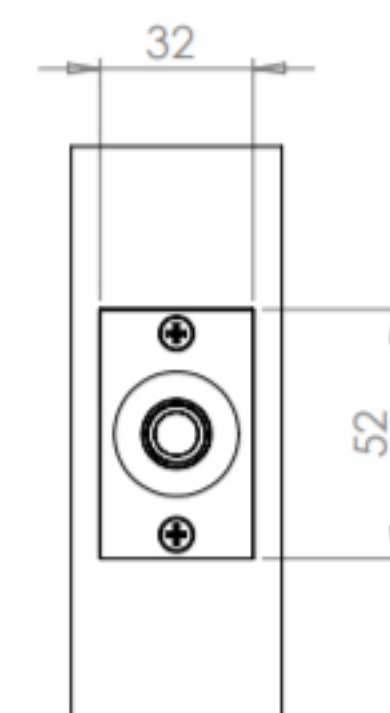
Face Plate Standard Width, Square
