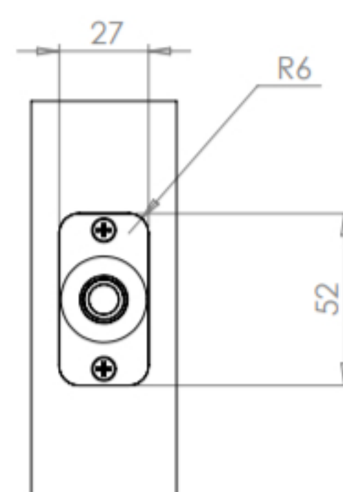
Face Plate Narrow Width, Radius
